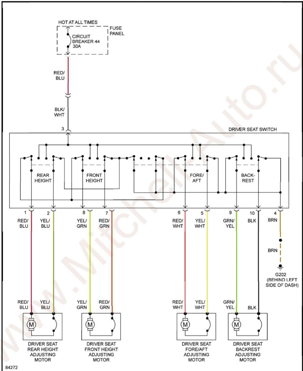
Fig. 28: Left Power Seat Circuit
