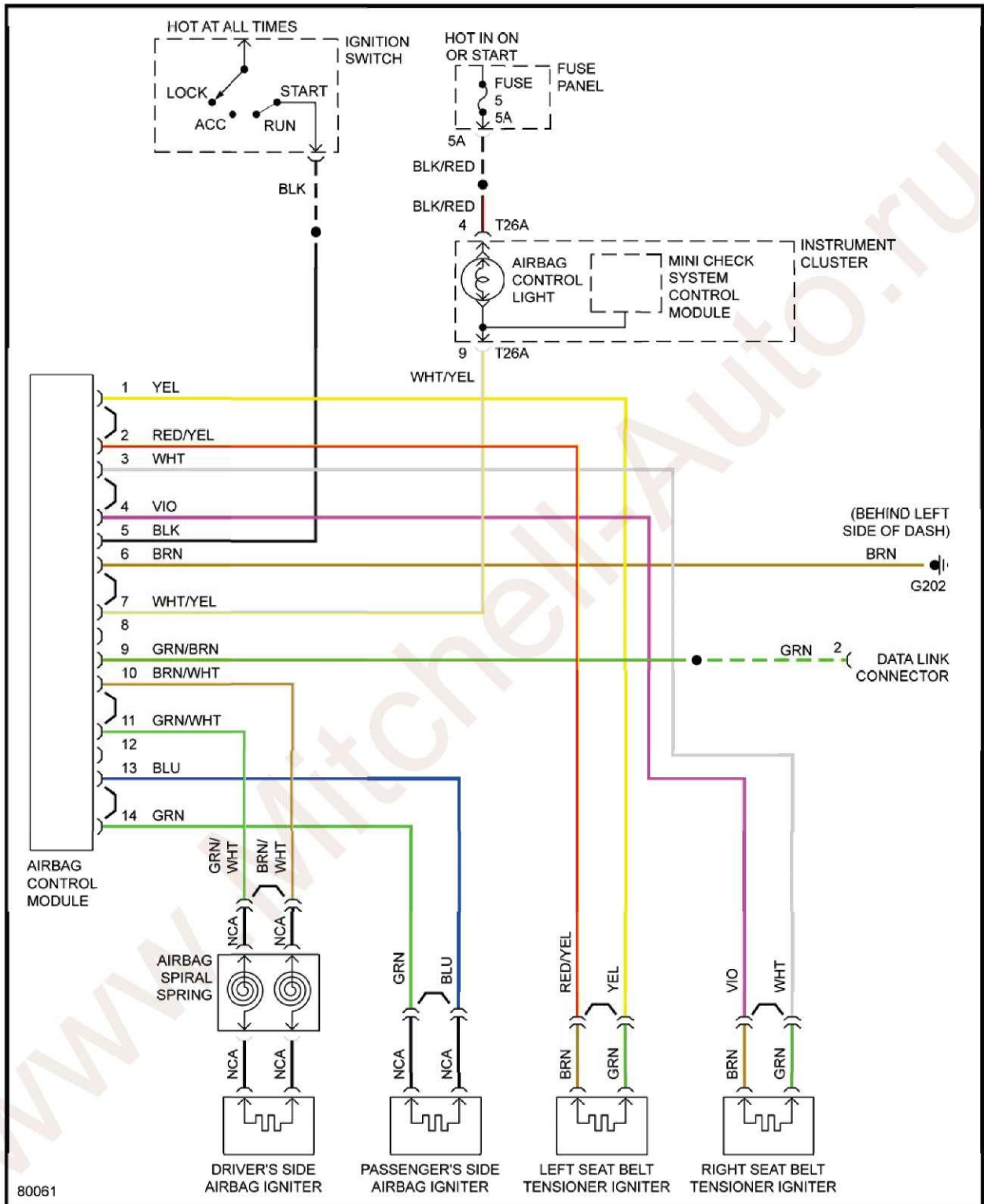
Fig. 36: Supplemental Restraints Circuit
