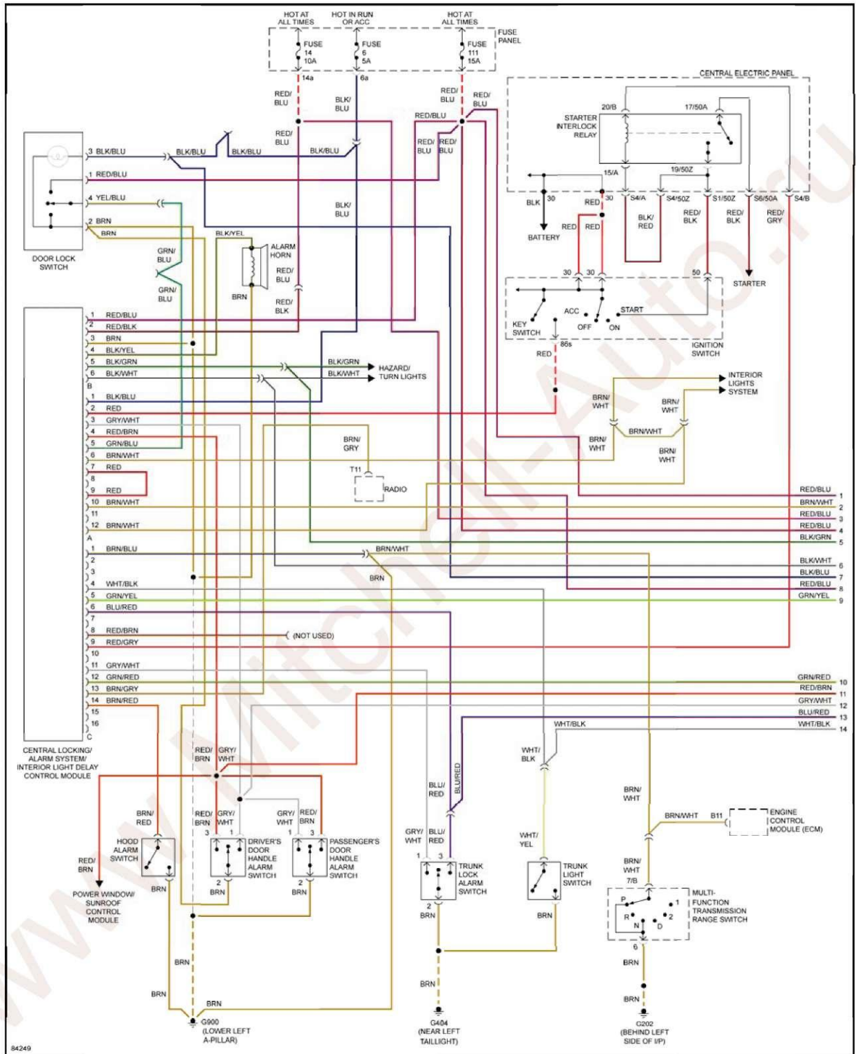
Fig. 5: Anti-theft & Central Locking Circuit (1 of 2)
