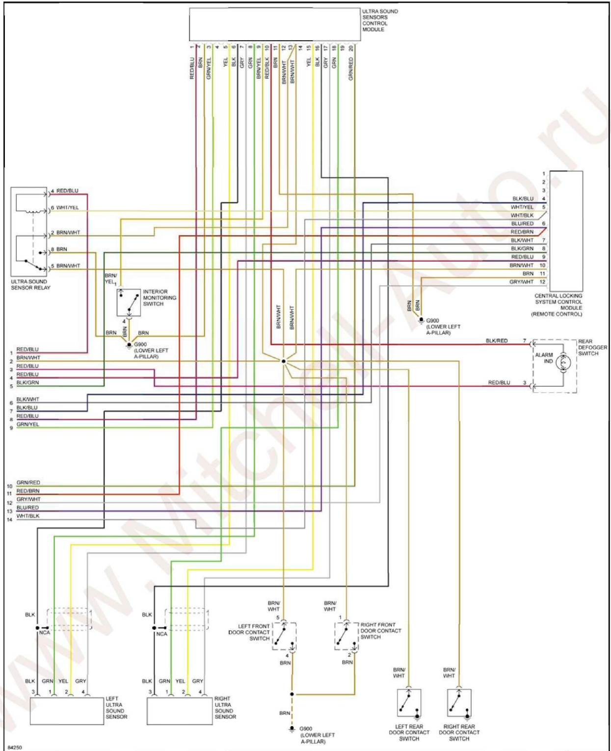
Fig. 6: Anti-theft & Central Locking Circuit (2 of 2)
