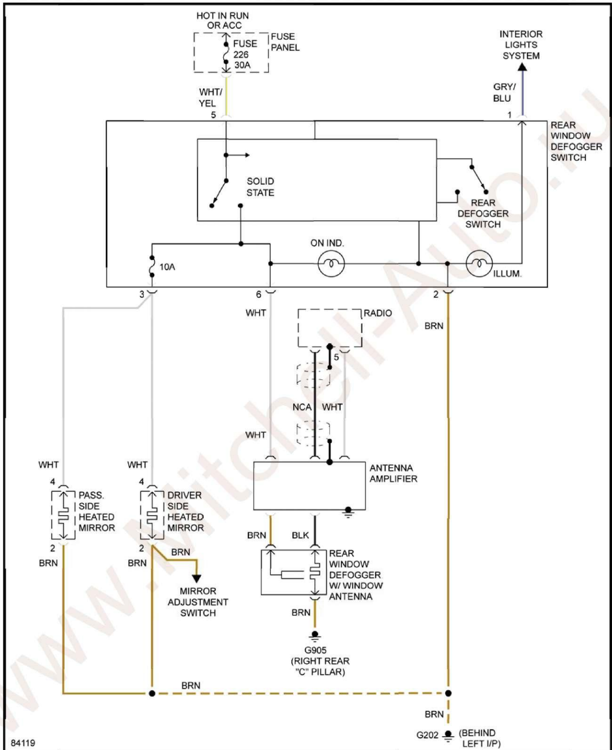
Fig. 10: W/ Antenna Amplifier Circuit
