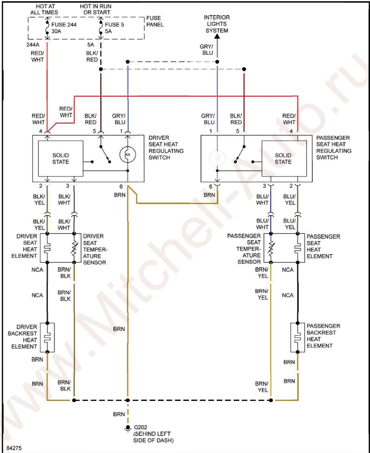
Fig. 27: Heated Seats Circuit
