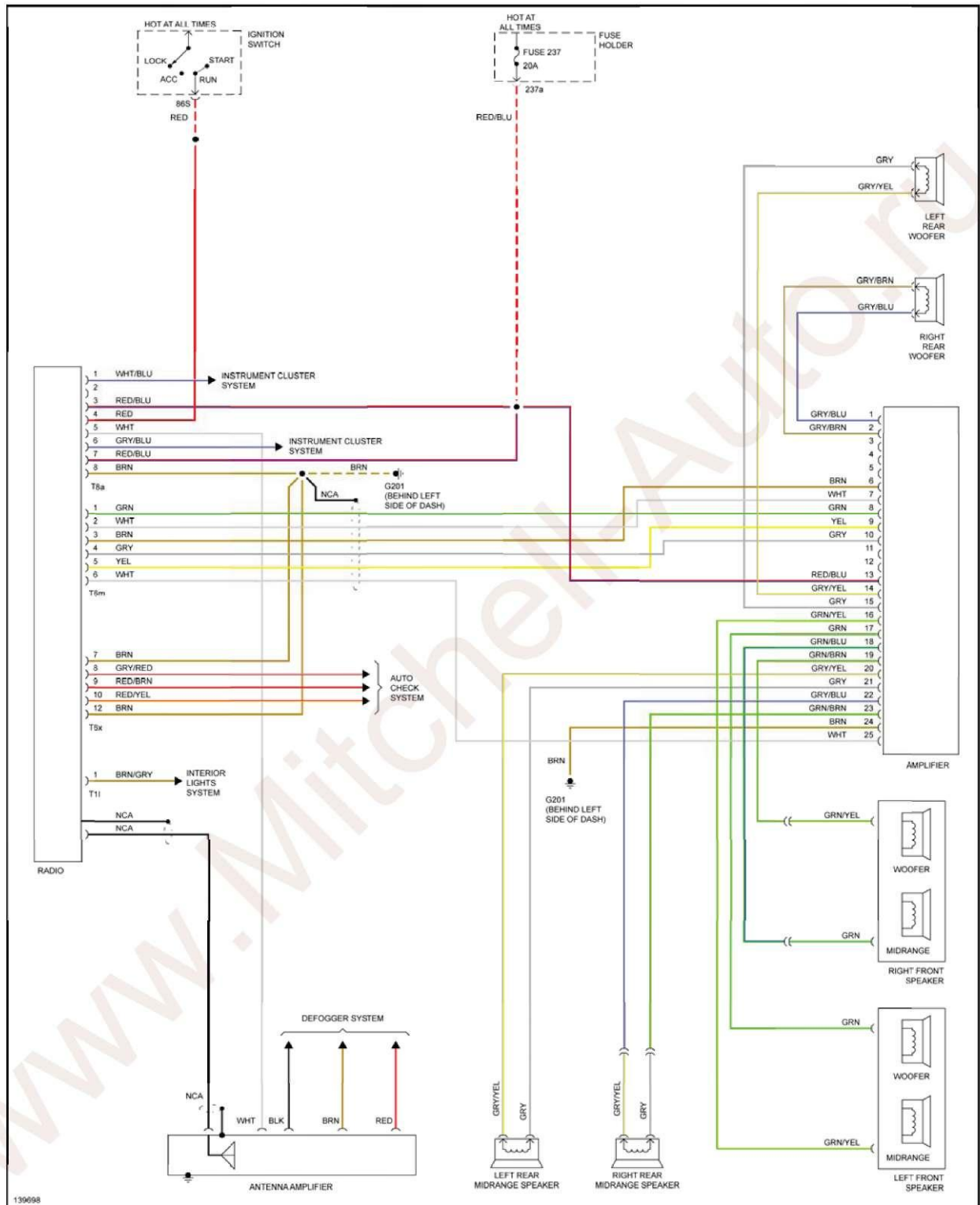
Fig. 32: Radio Circuit
