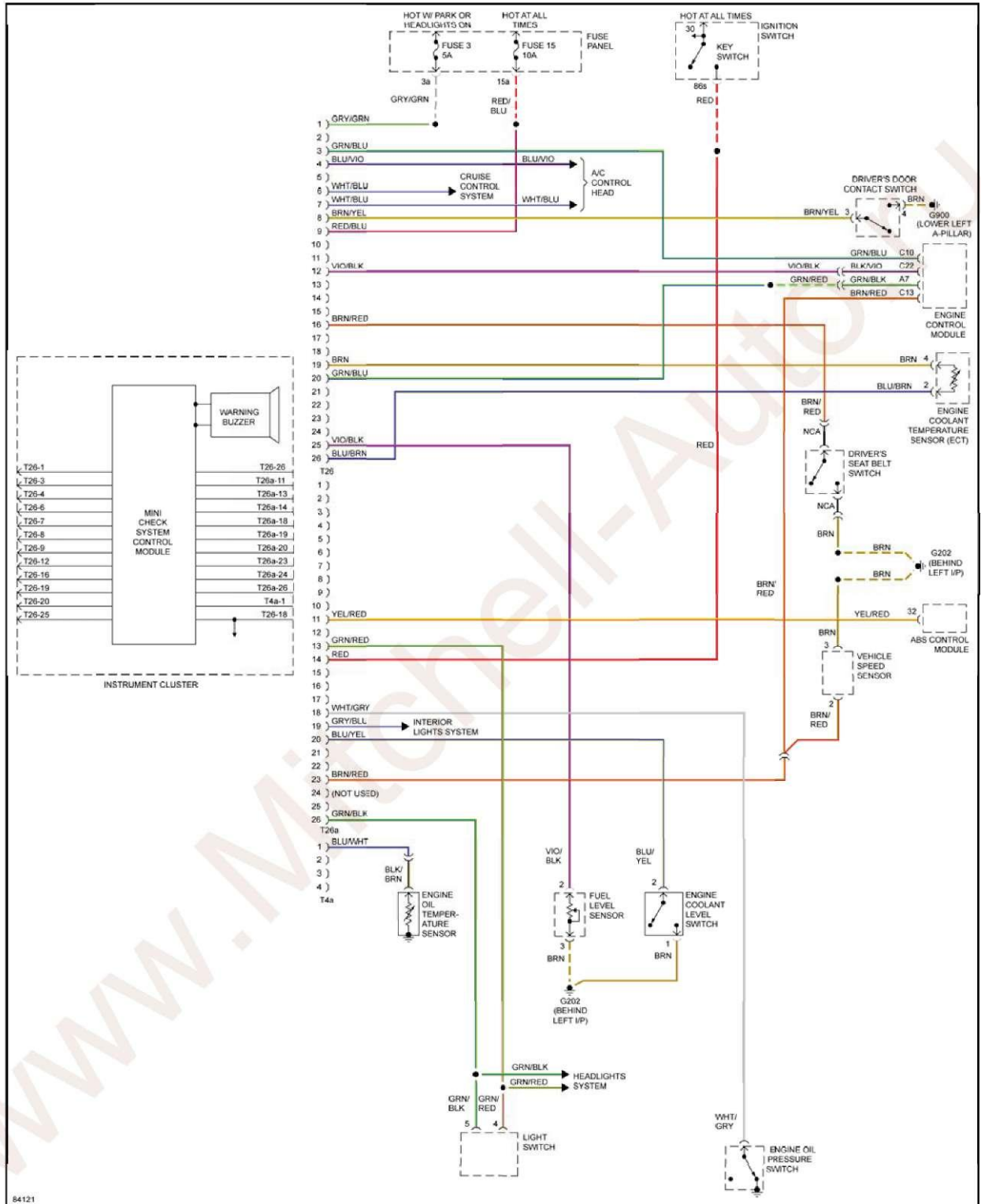
Fig. 38: Warning Systems Circuit
