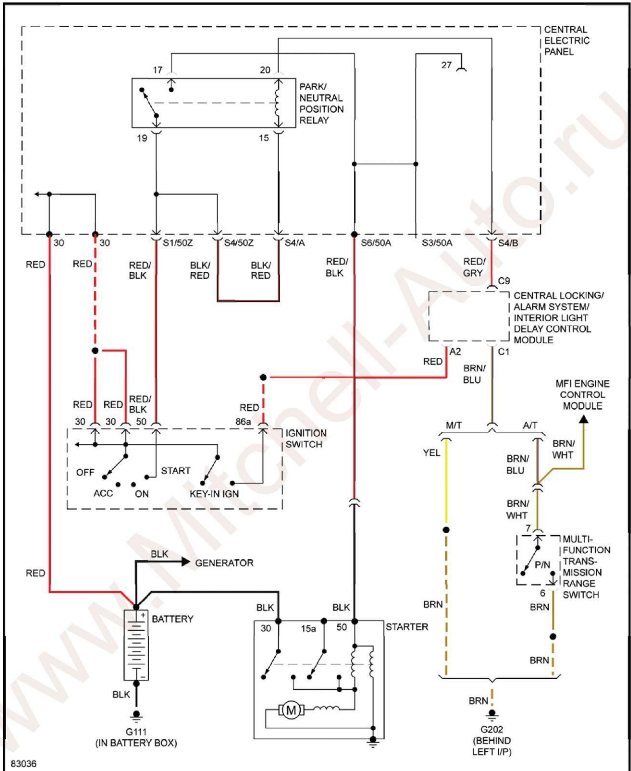
Fig. 35: Starting Circuit
