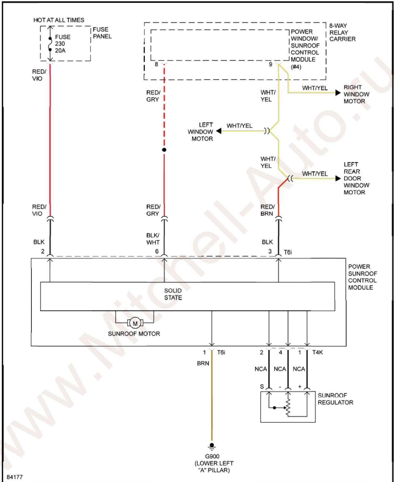
Fig. 29: Sunroof Circuit
