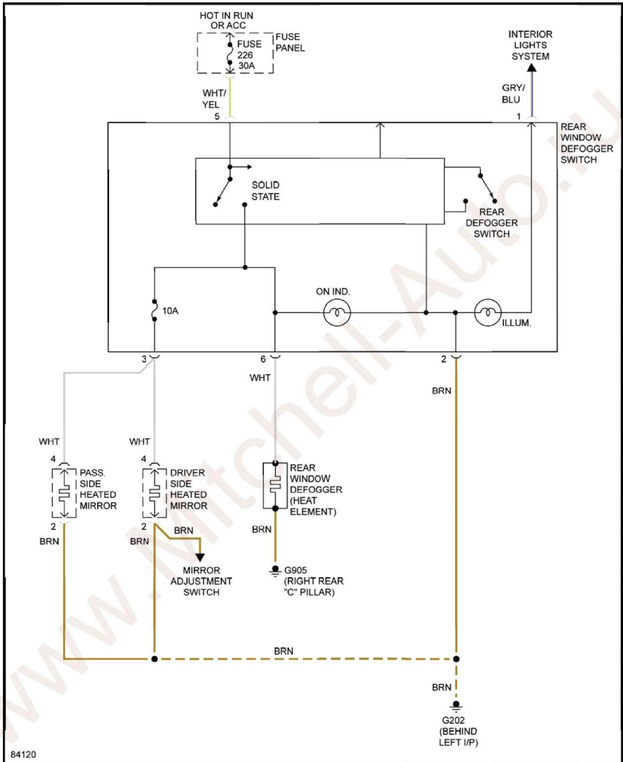
Fig. 11: W/O Antenna Amplifier Circuit
