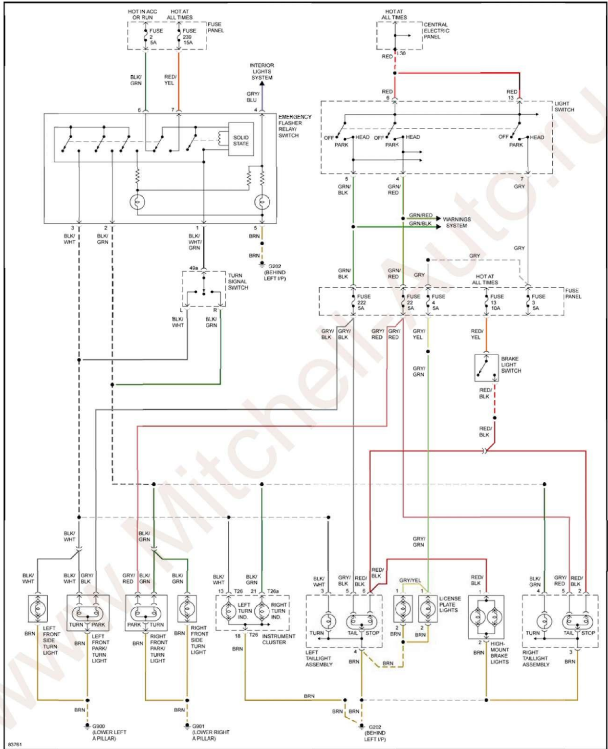
Fig. 15: Exterior Lamps Circuit
