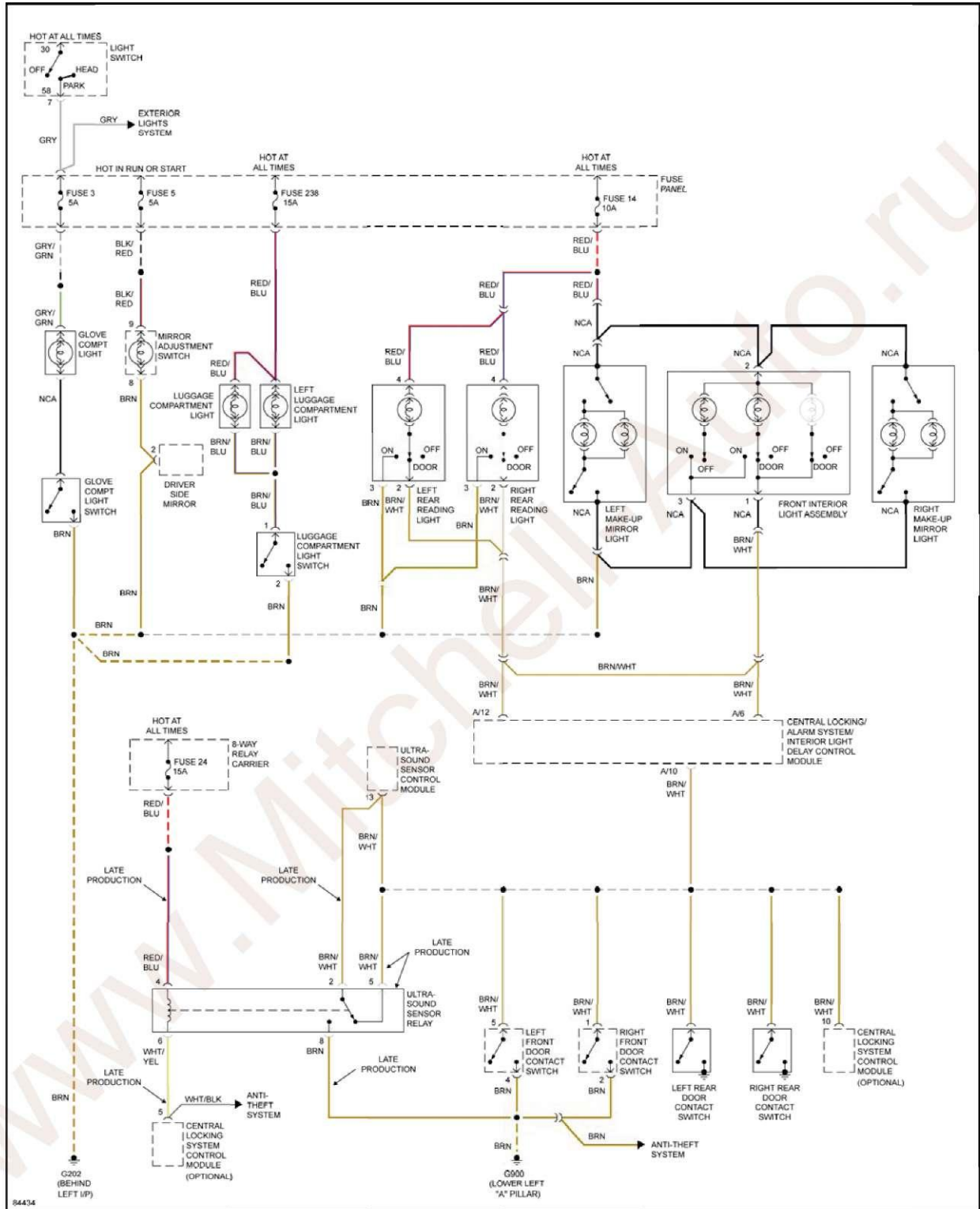
Fig. 21: Courtesy Lamps Circuit
