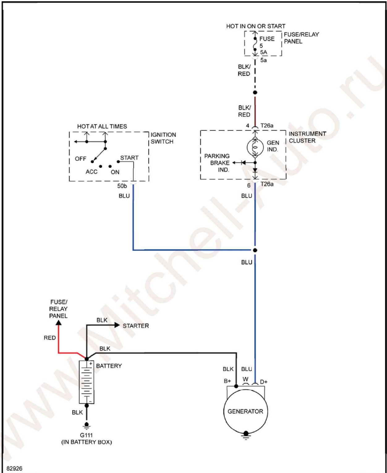
Fig. 34: Charging Circuit
