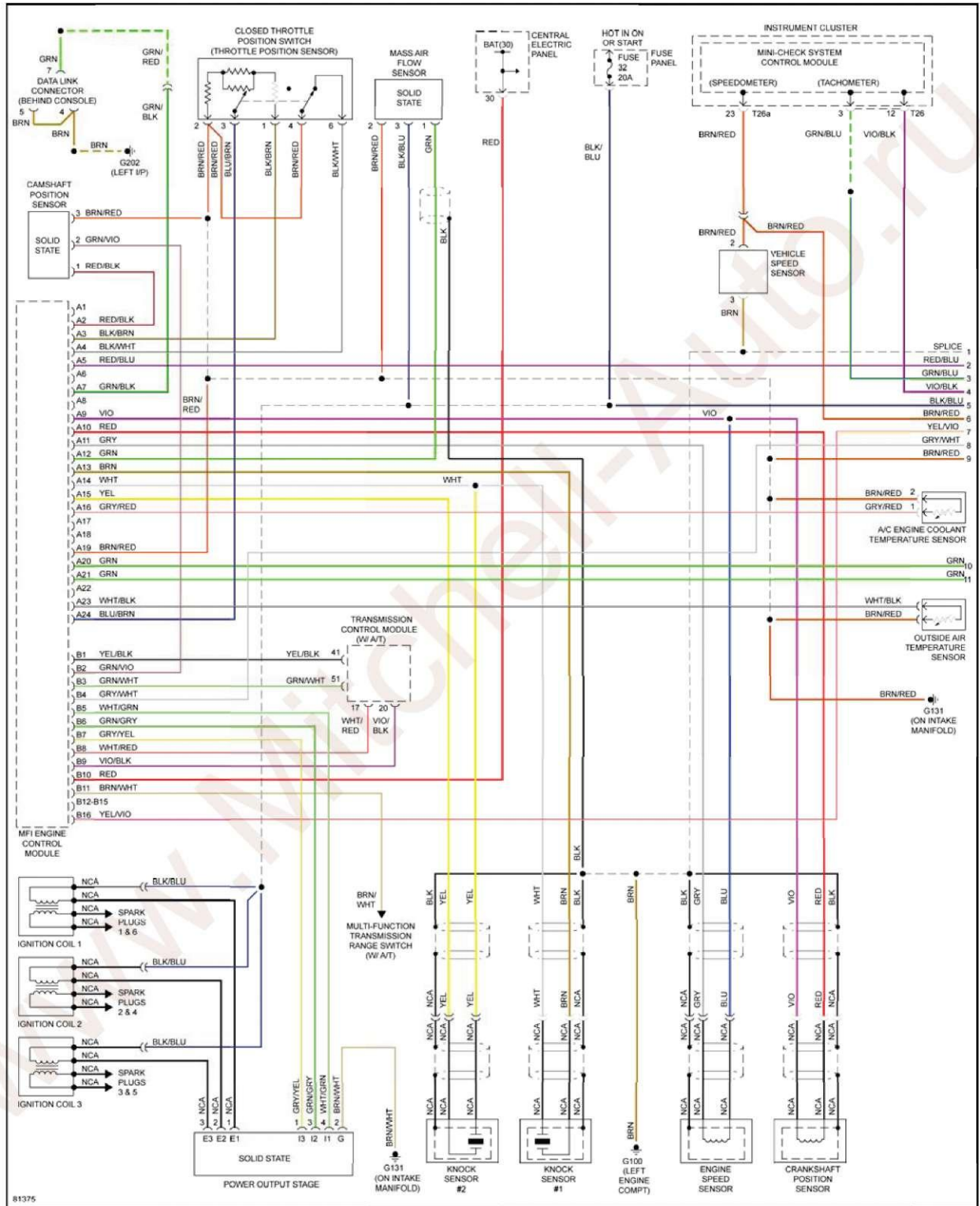
Fig. 12: 2.8L, Wiring Diagram (A4 2.8L Circuit 1 Of 2)
