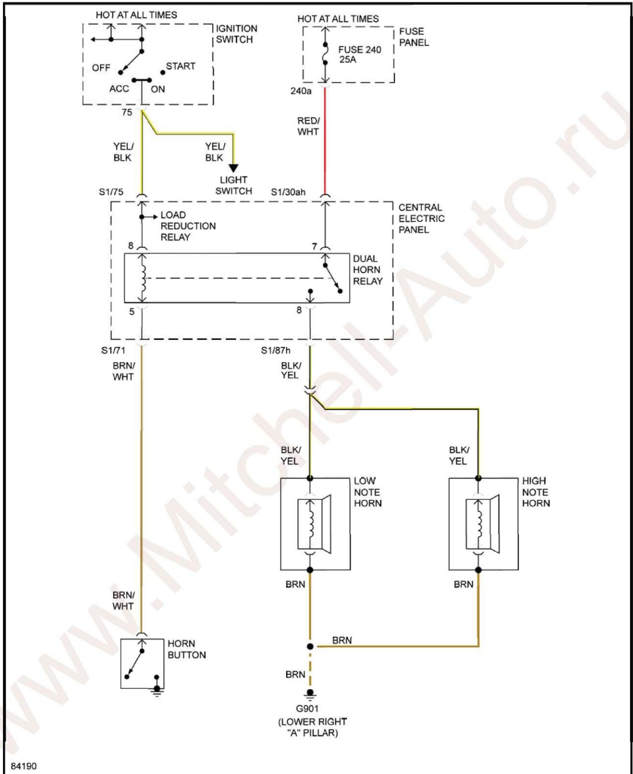
Fig. 19: Horn Circuit
